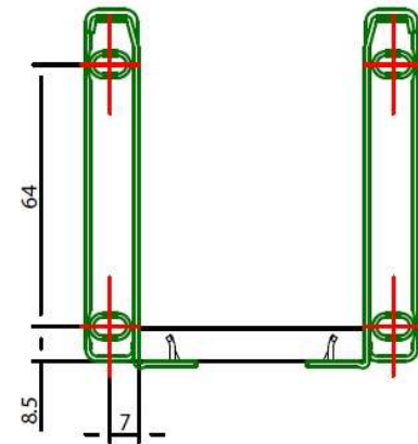
Installation dimensions of front connector
