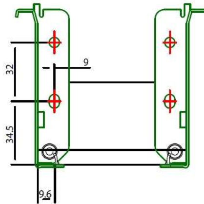
Back Panel Installation Dimensions
