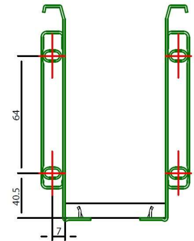
Installation dimensions of front connector
