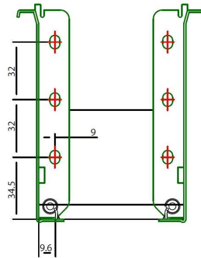
Back panel installation dimensions
